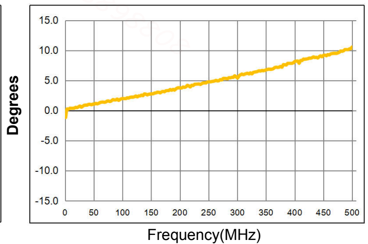
Phase Unbalance
