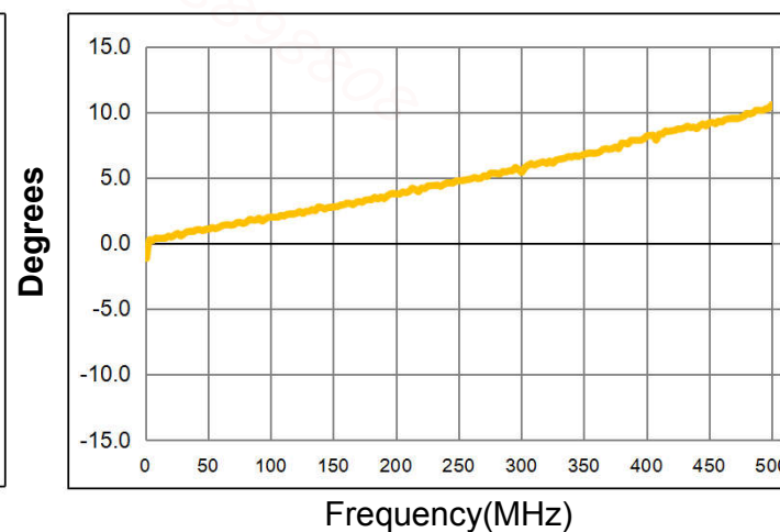
Phase Balance
