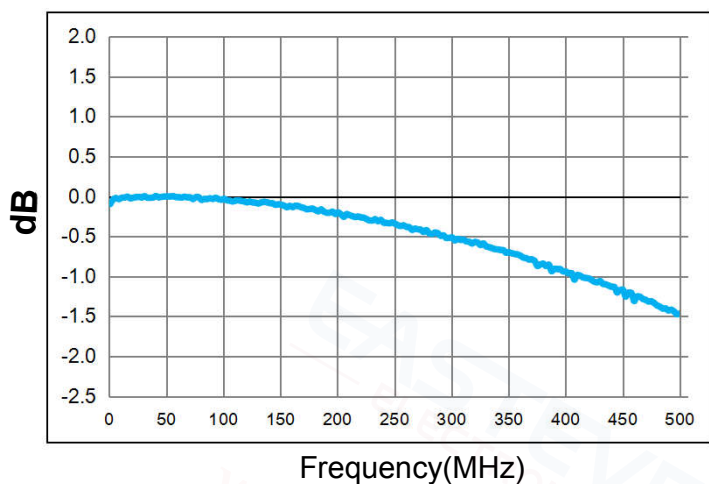
Amplitude Balance
